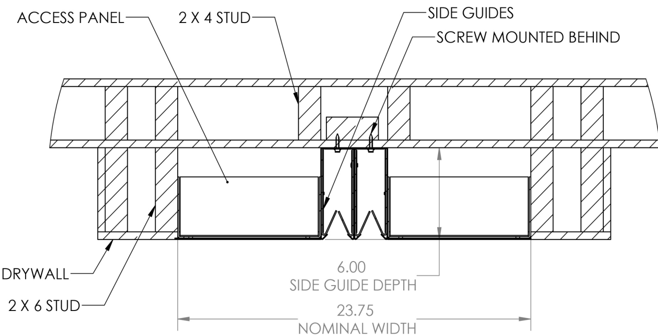
DEEP WALL MOUNT
