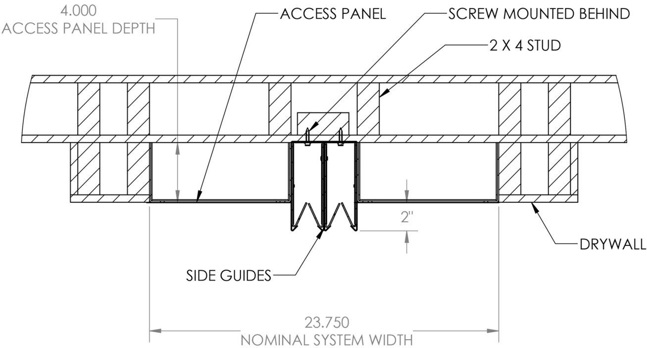
FALSE WALL MOUNT
