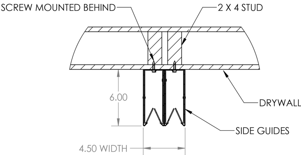
WALL SURFACE MOUNT
