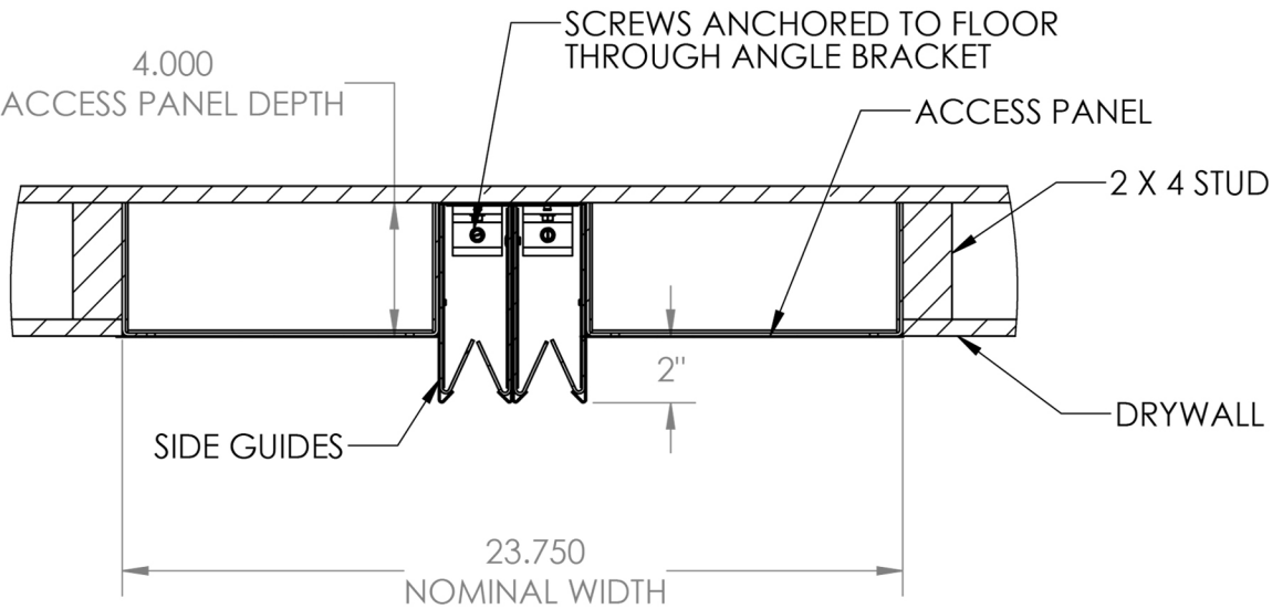
STANDARD WALL MOUNT
