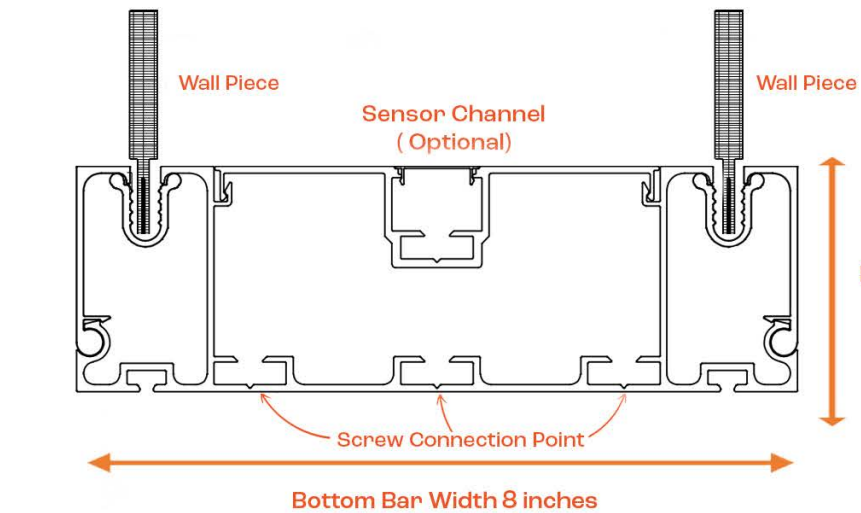
Dual Connected Bottom Bar
