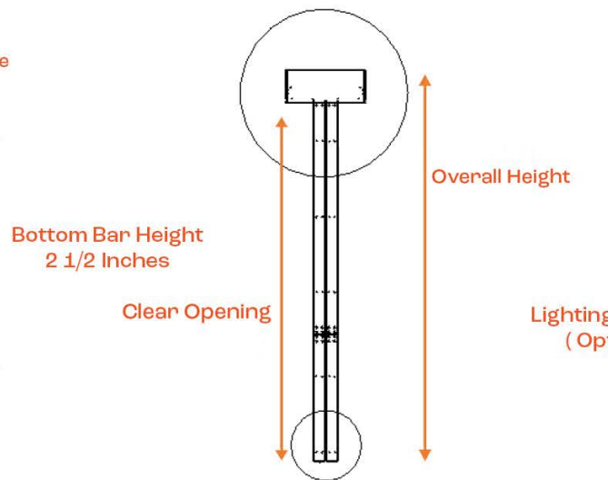
Side View of System
